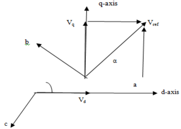
Fig.4: Voltage Space Vector and its Components
