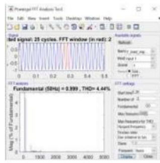
THD in Sag with D-STATCOM & SVPWM technique
