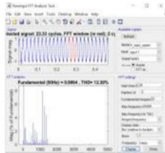
THD in Swell without D-STATCOM
