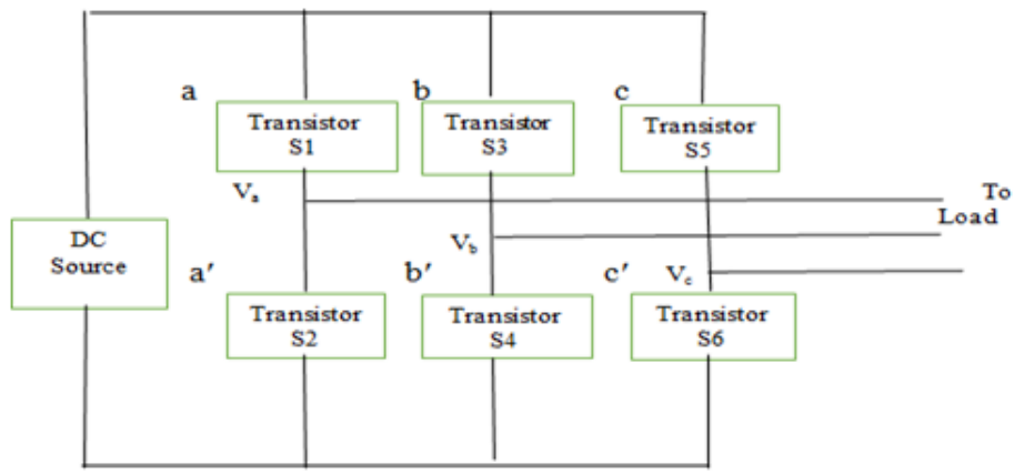
Fig.2 STATCOM Inverter
