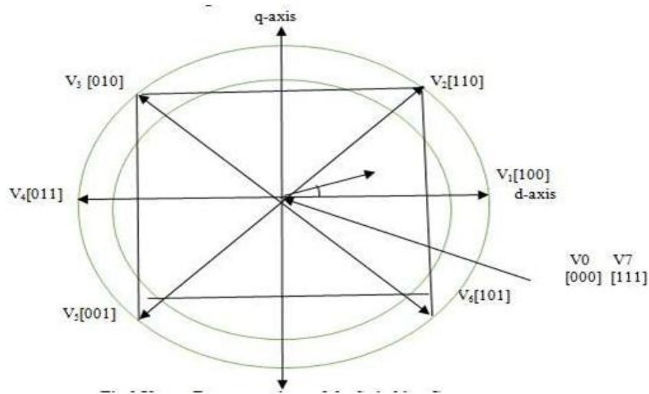
Fig.3 Vector Representations of the Switching Gate
