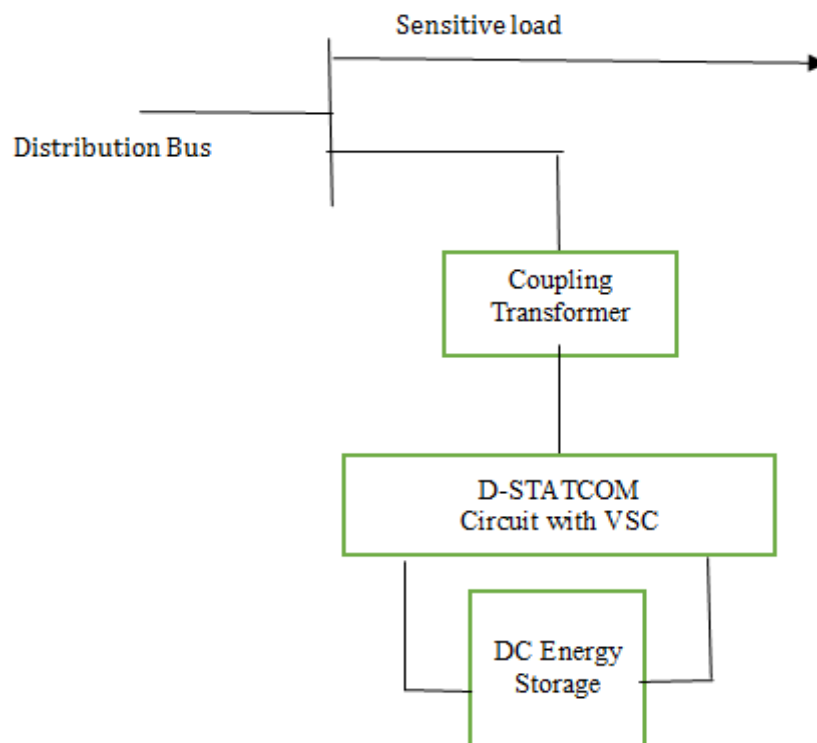
Fig.1: Constructional block diagram of D-STATCOM Operation of D-STATCOM
