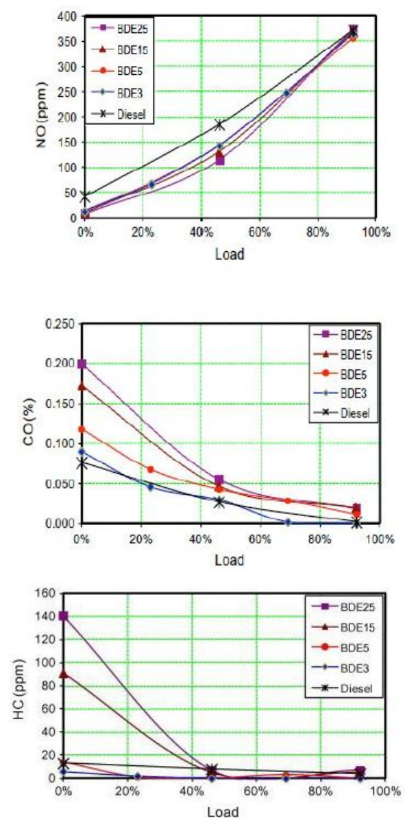
Fig. 1: Effect of diesel-biodiesel-ethanol blends on NO, CO and HC [11]
